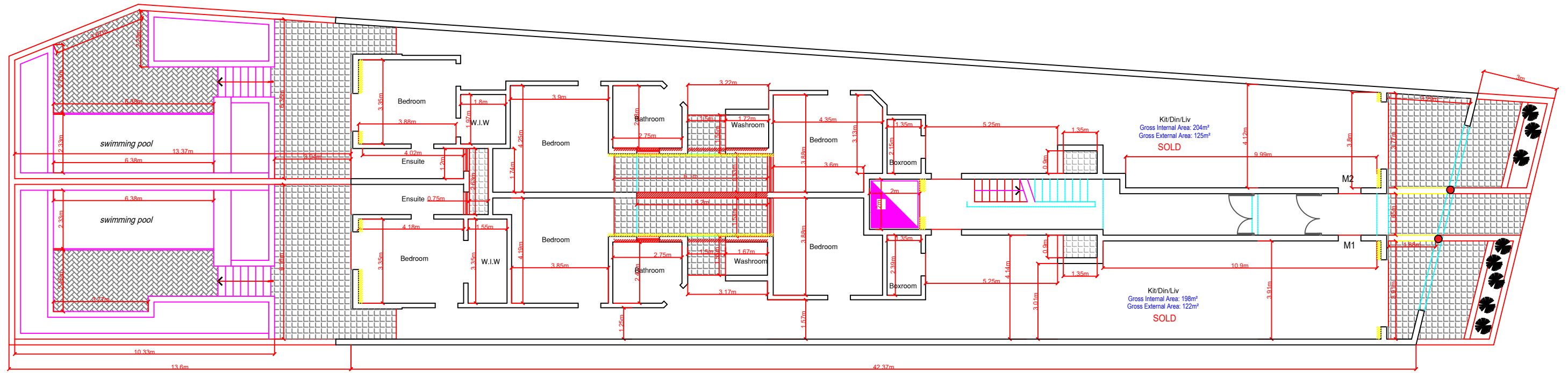
Proposed Ground Floor
