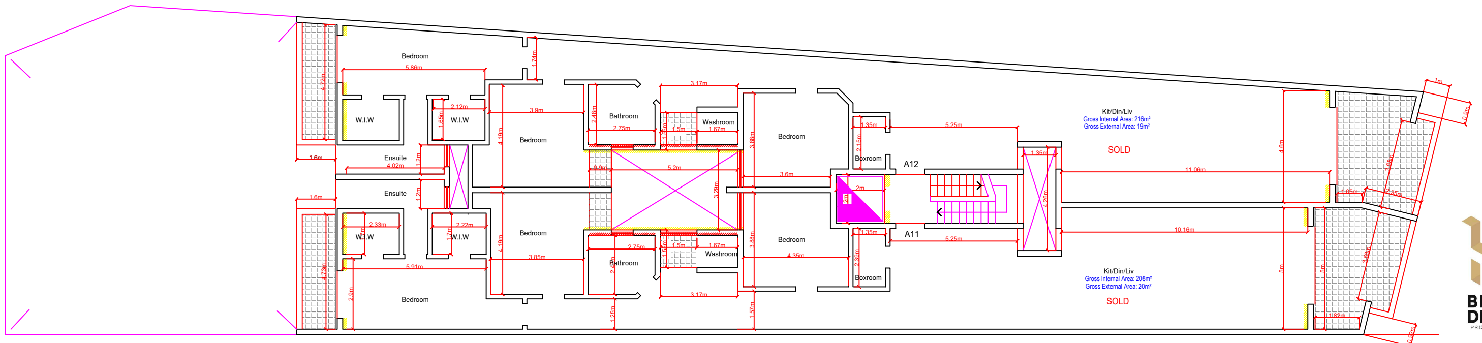
Proposed Sixth Floor
