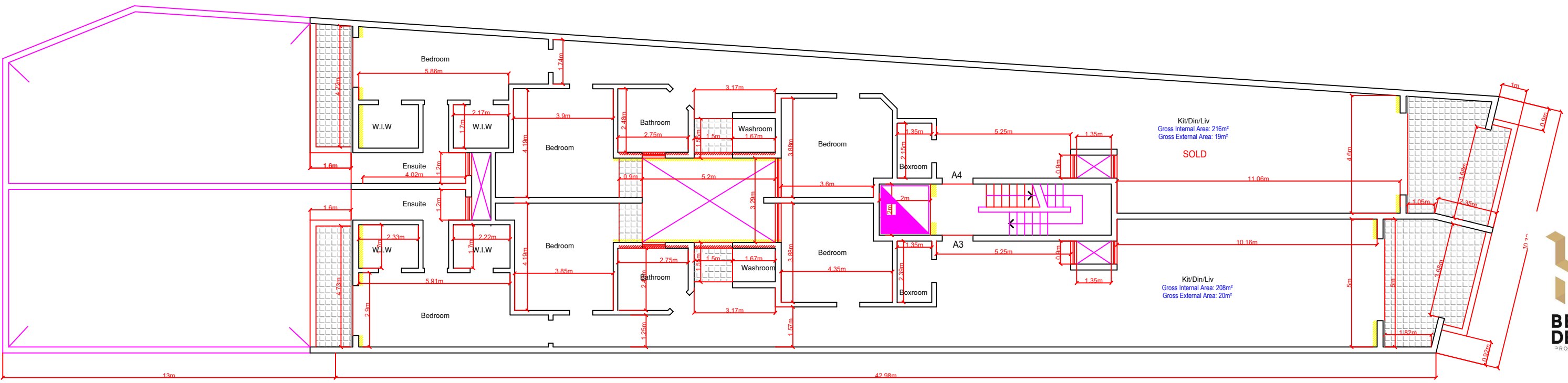
Proposed Second Floor
