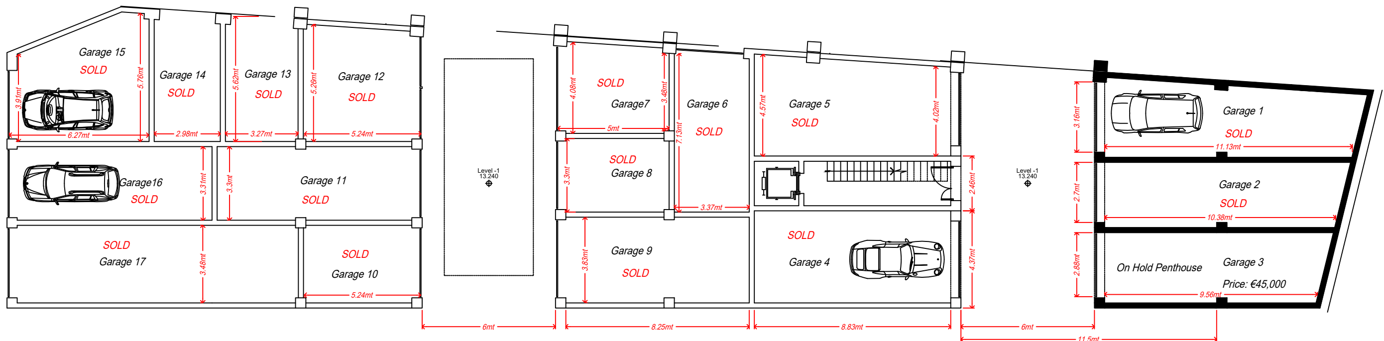
Proposed Basement.
